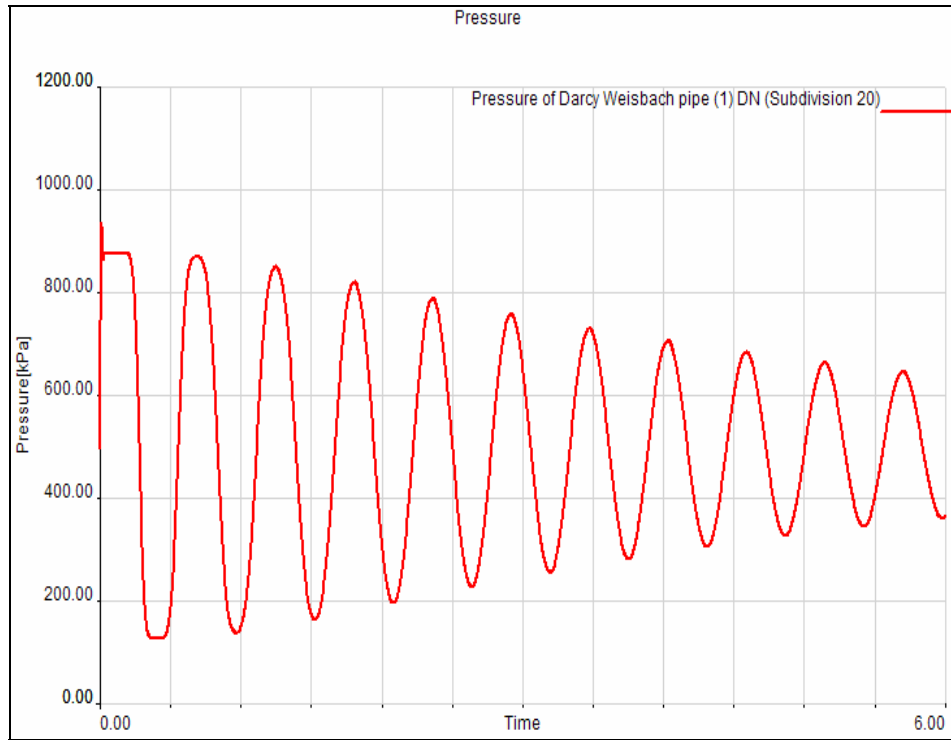
Figure 3: Water hammer simulation results.
