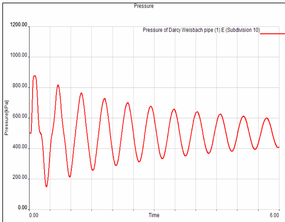
Figure 4: Water hammer simulation results.
